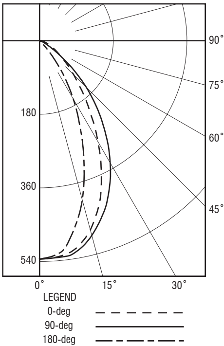
C2W-L16 Wallwash- Polar Diagram
