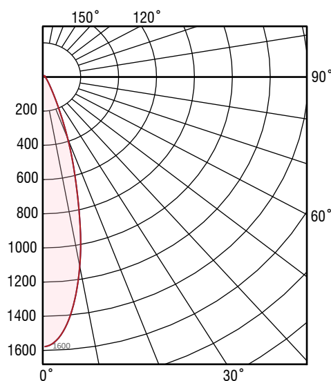
C20-L10 35° Optic, 6500K - Polar Diagram
