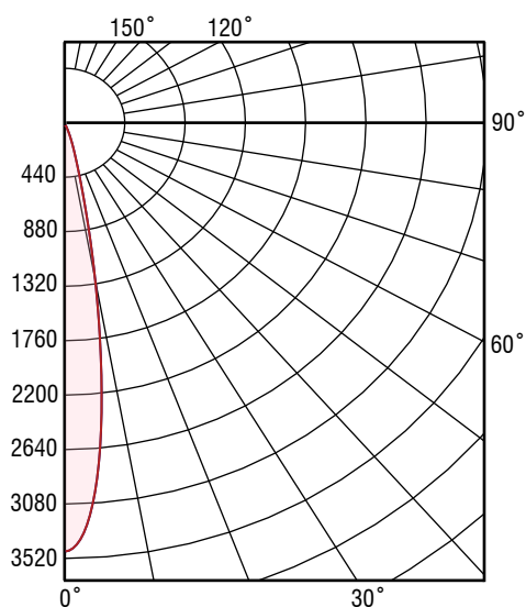
C20-L10 15° Optic, 6500K - Polar Diagram
