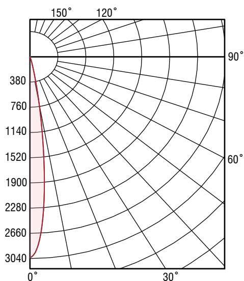
C20-L10 15° Optic, 2700K - Polar Diagram
