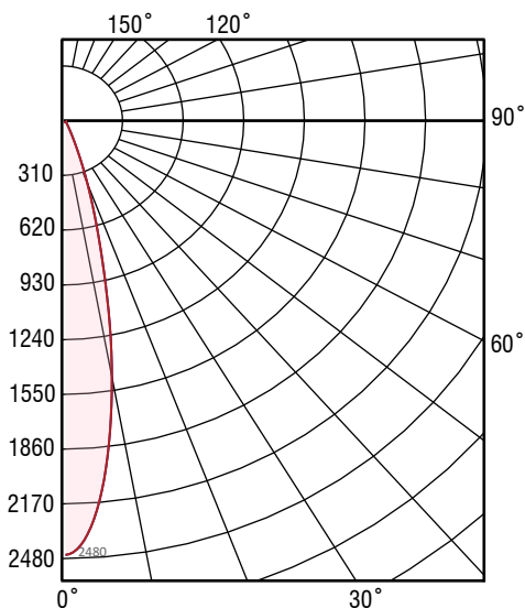
C20-L10 25° Optic, 6500K - Polar Diagram
