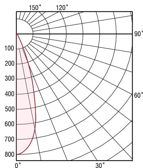
C20-L10 35° Optic, 2700K - Polar Diagram
