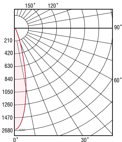
C20-L10 25° Optic, 2700K - Polar Diagram
