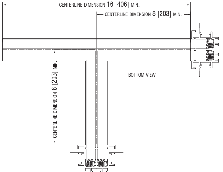
REFLECTED CEILING PLAN VIEW:
