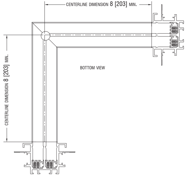
ELBOW SPLICE BOX FEED ELBOW FEED
