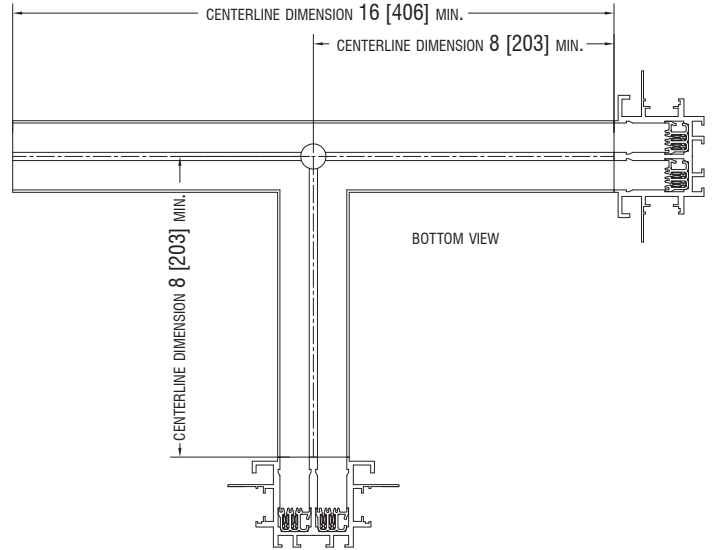
ELBOW SPLICE BOX FEED ELBOW FEED
