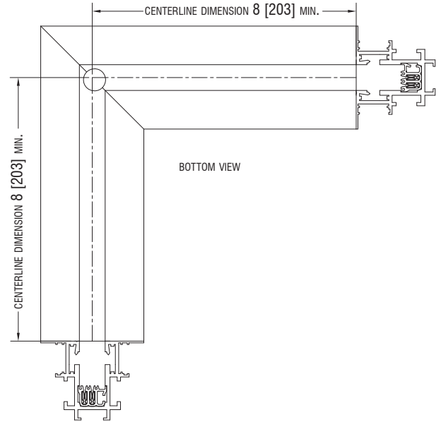
ELBOW SPLICE BOX FEED ELBOW FEED
