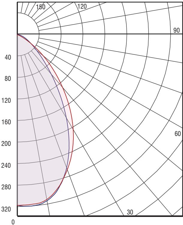
A3W-L10, 2700K Wallwash - Polar Plot of Candela
