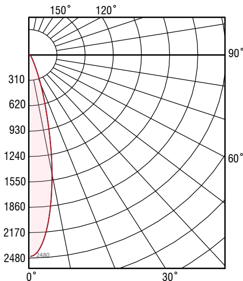
A30-L10 25° Optic, 6500K - Polar Diagram
