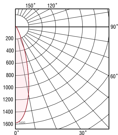
A30-L10 35° Optic, 6500K - Polar Diagram
