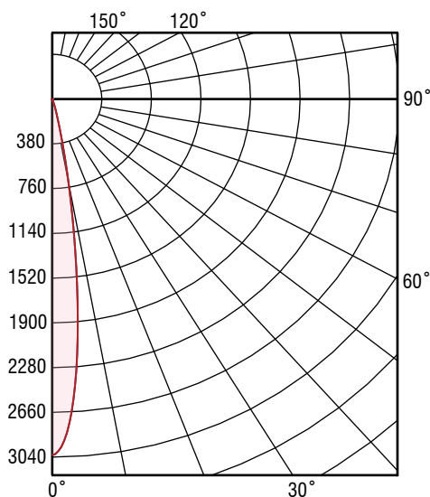
A30-L10 15° Optic, 2700K - Polar Diagram
