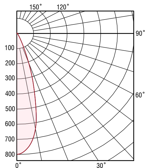
A30-L10 35° Optic, 2700K - Polar Diagram
