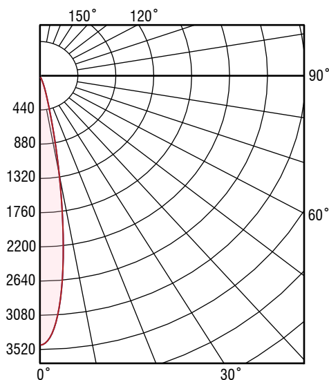
A30-L10 15° Optic, 6500K - Polar Diagram
