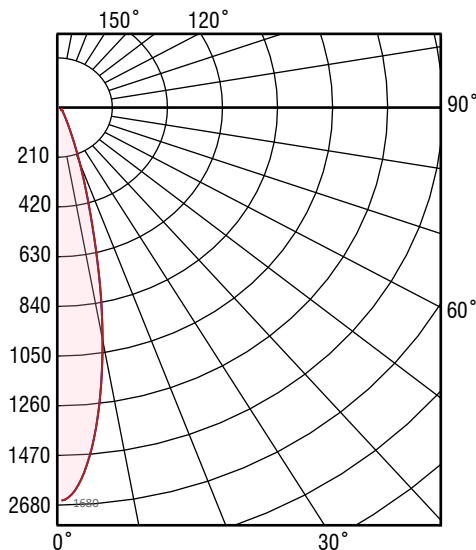
A30-L10 25° Optic, 2700K - Polar Diagram
