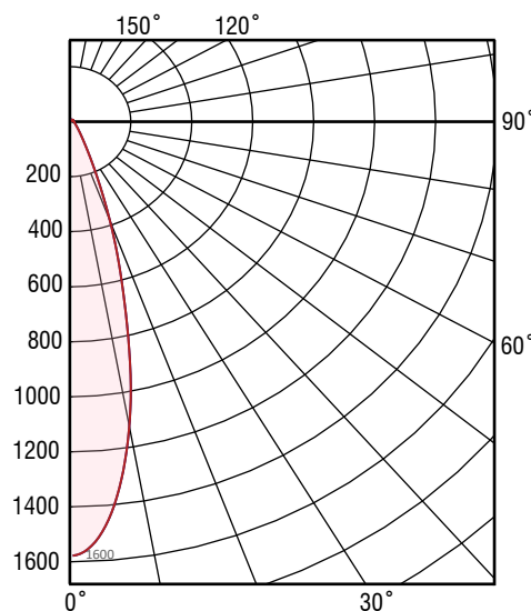
A30-L10 35° Optic, 6500K - Polar Diagram
